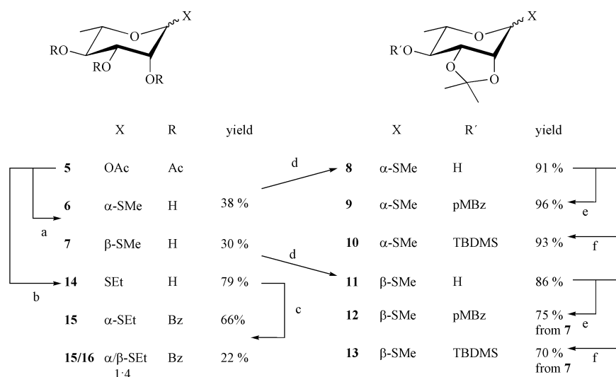
Scheme 2 Reagents and conditions: a: 1) TMSSMe, TMSOTf, \text{CH}_2\text{Cl}_2 , Ar, 0^\circ\text{C} \rightarrow \text{rt} ; 2) NaOMe–MeOH; b: 1) EtSH, \text{BF}_3 \cdot \text{OEt}_2 , \text{CH}_2\text{Cl}_2 , Ar, 0^\circ\text{C} \rightarrow \text{rt} ; 2) NaOMe–MeOH; c: benzoyl chloride, pyridine, DMAP (cat.) over night, 0^\circ\text{C} \rightarrow \text{rt} ; d: dimethoxypropane, \text{CH}_2\text{Cl}_2 , TosOH (cat.); e: pMBzCl, pyridine, \text{CH}_2\text{Cl}_2 , 0^\circ\text{C} \rightarrow \text{rt} ; f: TBDMSCl, DMF, imidazole.
