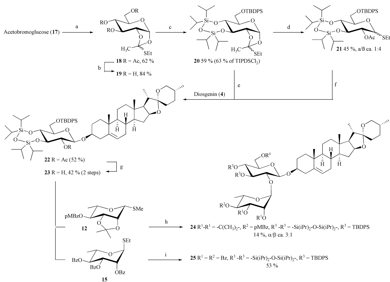
Scheme 3 Reagents and conditions: a: EtSH, sym -collidine, \text{NBu}_4\text{Br} , anhydr. acetonitrile; b: NaOMe–MeOH; c: 1) TBDPSCl, 12 h; 2) TIPDS \text{Cl}_2 (0.95 eq.), 6 h, 0^\circ\text{C} \rightarrow \text{rt} , argon, imidazole, DMF; d: EtSH, abs. \text{CH}_2\text{Cl}_2 , Ar, TMSOTf (cat.), MS 4 \text{\AA} , rt, 5 min; e: anhydr. \text{Et}_2\text{O}-\text{CH}_2\text{Cl}_2 1 : 1, argon, MS 4 \text{\AA} ; 1) NIS, 2 h; 2) TFOH (cat.), 2 h; f: DMTST, \text{CH}_2\text{Cl}_2 , MS 4 \text{\AA} , 24 h; g: \text{K}_2\text{CO}_3 –MeOH; h: NIS, anhydr. \text{Et}_2\text{O}-\text{CH}_2\text{Cl}_2 1 : 1, argon, MS 4 \text{\AA} ; i: DMTST, \text{Et}_2\text{O} , MS 4 \text{\AA} .
